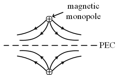
Figure 32.9: On a PEC surface, the requisite boundary condition is \hat{n} \cdot \mathbf{B} = 0 . Hence, a magnetic monopole on top of a PEC surface will have magnetic field distributed as shown. By image theory, such a distribution of the \mathbf{B} field can be obtained by adding a magnetic monopole of the same polarity at its image point.
